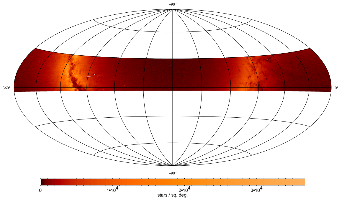
Figure 1: This shows the density of stars in CMC13.
