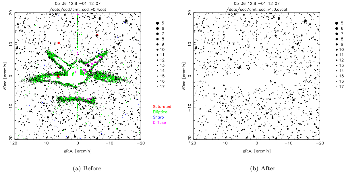
Figure 8: This figure shows the area around Epsilon Orionis (Alnilam) a 1.7 magnitude star, before and after the bright star mask has been applied.
