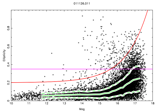
Figure 6: This plot shows the magnitude-dependent ellipticity limits (red line) used in the survey. Also shown is the old constant limit (magenta line) which caused many faint stars to be flagged needlessly. The green lines show the median and width (equivalent to a Gaussian sigma) of the ellipticity distribution.
