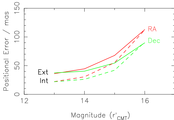
Figure 9: The internal and external positional errors as a function of magnitude. The solid line gives the median external errors and the dashed line shows the equivalent internal errors. RA is shown in red and declination in green.
