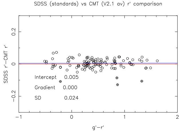
Figure 4: The residuals in r' between the SDSS standards and CMT as a function of colour.
