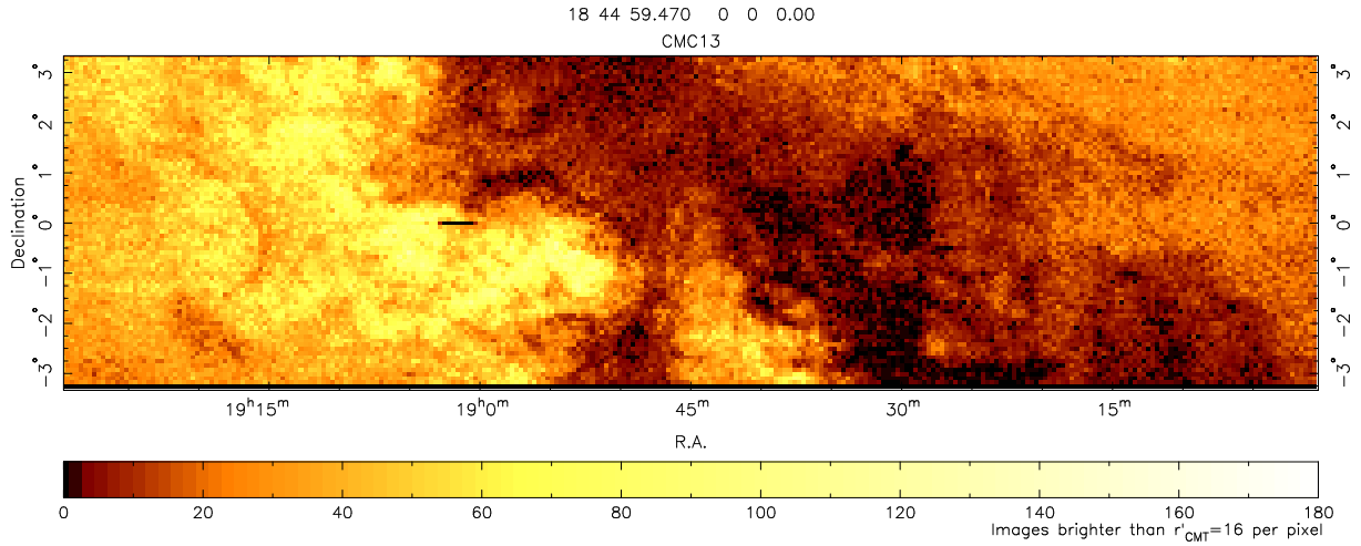
Figure 5: This shows the density variations crossing the Galactic plane. The black stripe is one of the 23 holes in the catalogue mentioned in the text.
