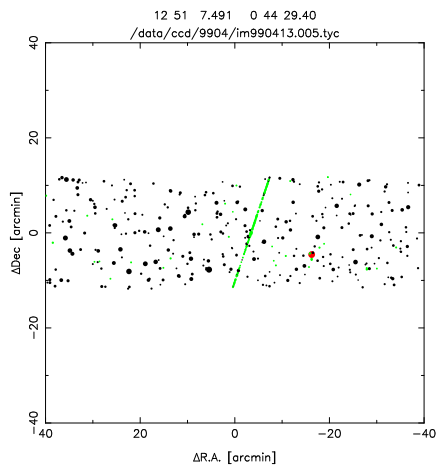
(a) Satellite trail
